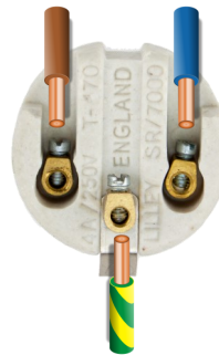
Metal Lampholder
