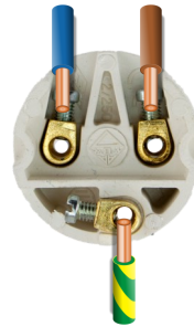
Metal Lampholder
